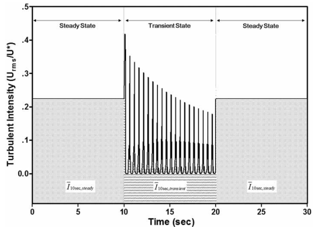
Figure 9 | Temporal variation of turbulence intensity over 10 seconds of a transient event at a point 5 m from the end valve.
