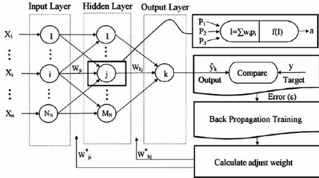
Figure 2 | A three-layered feed-forward neural network with the back propagation (BP) training algorithm.
